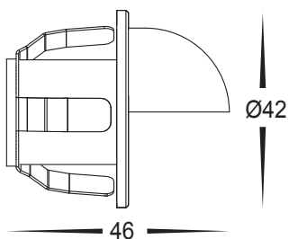
Cutout Ø30
